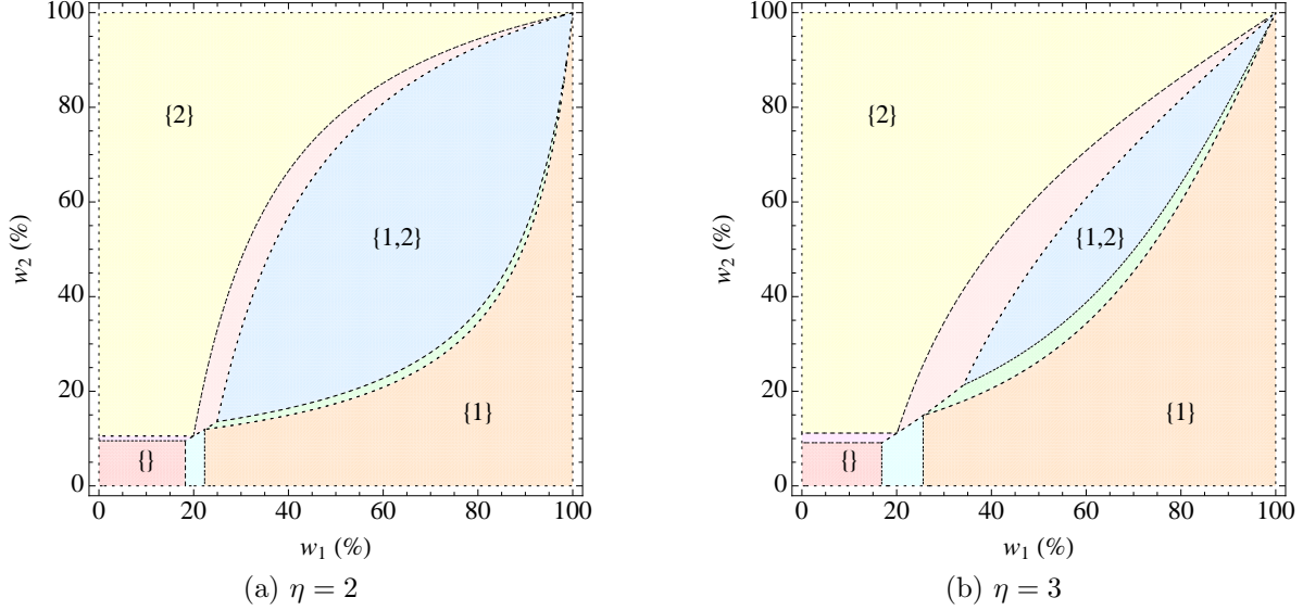
Figure 7: Modifying the example illustrated in Figure 2 to allow for partial alleviation with cost functions as in (24). There are two potential catastrophes, with \tau_1 = 20\% and \tau_2 = 10\% . Unnumbered zones are areas where one of the catastrophes should be partially alleviated (and it should be obvious from the location which one).
