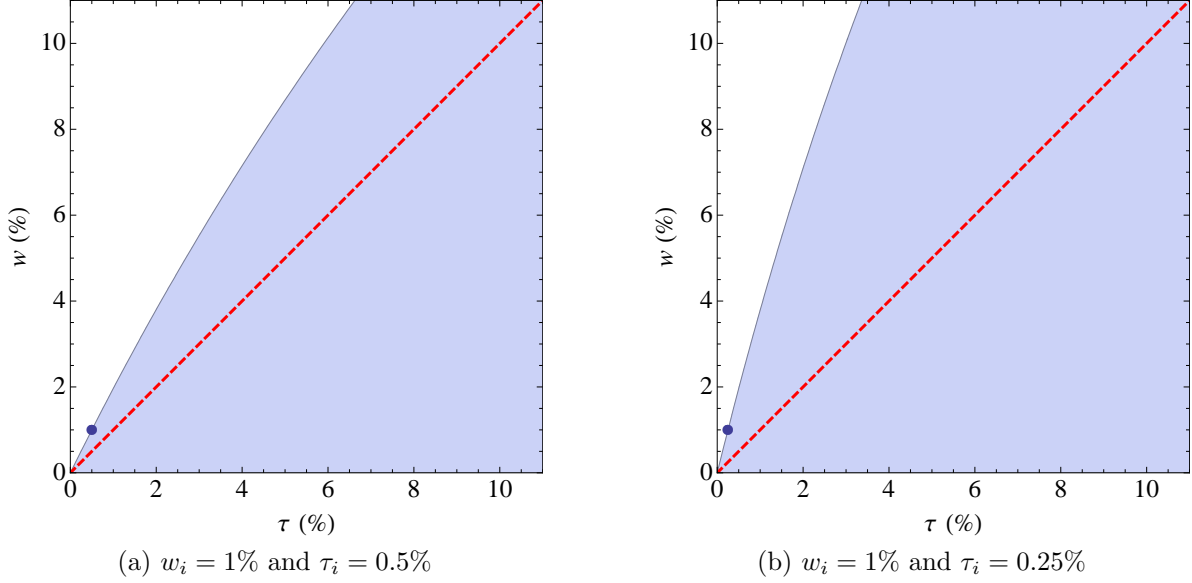
Figure 4: Illustration of Example 5. The presence of many small catastrophes (each with cost \tau_i and WTP w_i , indicated by a solid circle) expands the region of inaction for a larger catastrophe, which should not be averted if its cost \tau and WTP w lie in the shaded region.
