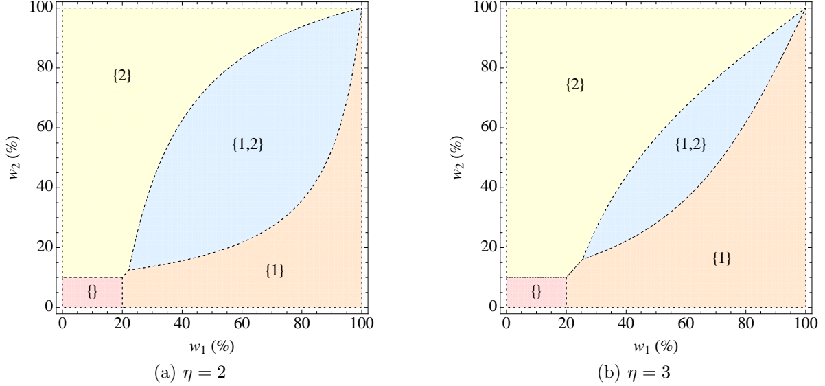
Figure 2: There are two potential catastrophes, with \tau_1 = 20\% and \tau_2 = 10\% . The figures show, for all possible values of w_1 and w_2 , which catastrophes should be averted (in curly brackets). A catastrophe for which w_i < \tau_i should not be averted. We should avert both catastrophes only for combinations (w_1, w_2) in the middle shaded region. That region shrinks considerably when risk aversion, \eta , increases.
