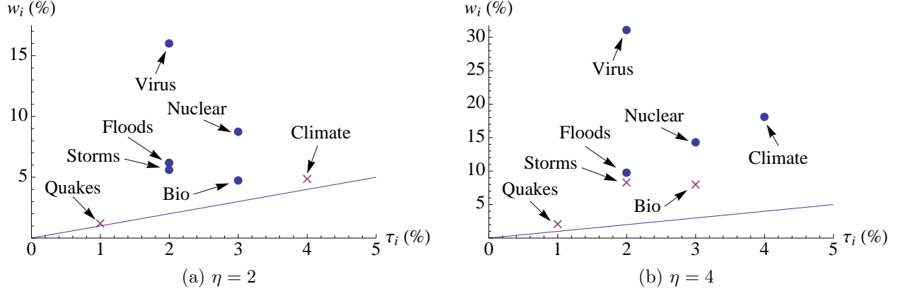
Figure 8: The figures show which of the seven catastrophes summarized in Table 1 should be averted. Catastrophes that should be averted are indicated by blue dots in each panel; catastrophes that should not be averted are indicated by red crosses.
