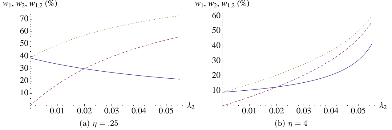
Figure 1: Effects of background risk: The figures fix \delta = .02, g = .02, \beta_1 = \beta_2 = 6, \lambda_1 = .02 , and plot w_1 (solid), w_2 (dashed), and w_{1,2} (dotted) for a range of values of \lambda_2 .
