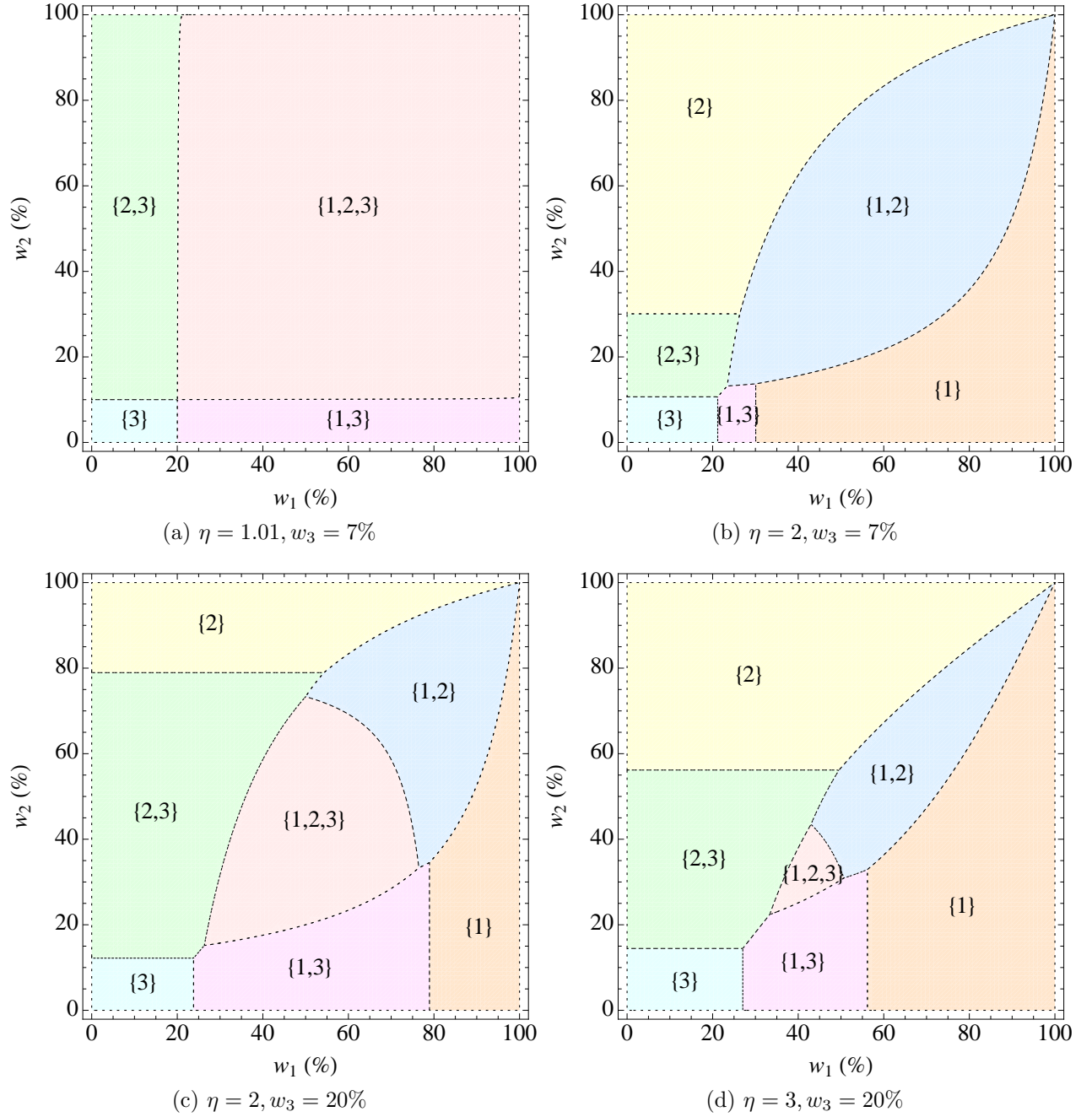
Figure 3: There are three catastrophe types with \tau_1 = 20\% , \tau_2 = 10\% , and \tau_3 = 5\% . Different panels make different assumptions about w_3 and \eta . Numbers in brackets indicate which catastrophes should be averted for different values of w_1 and w_2 .
