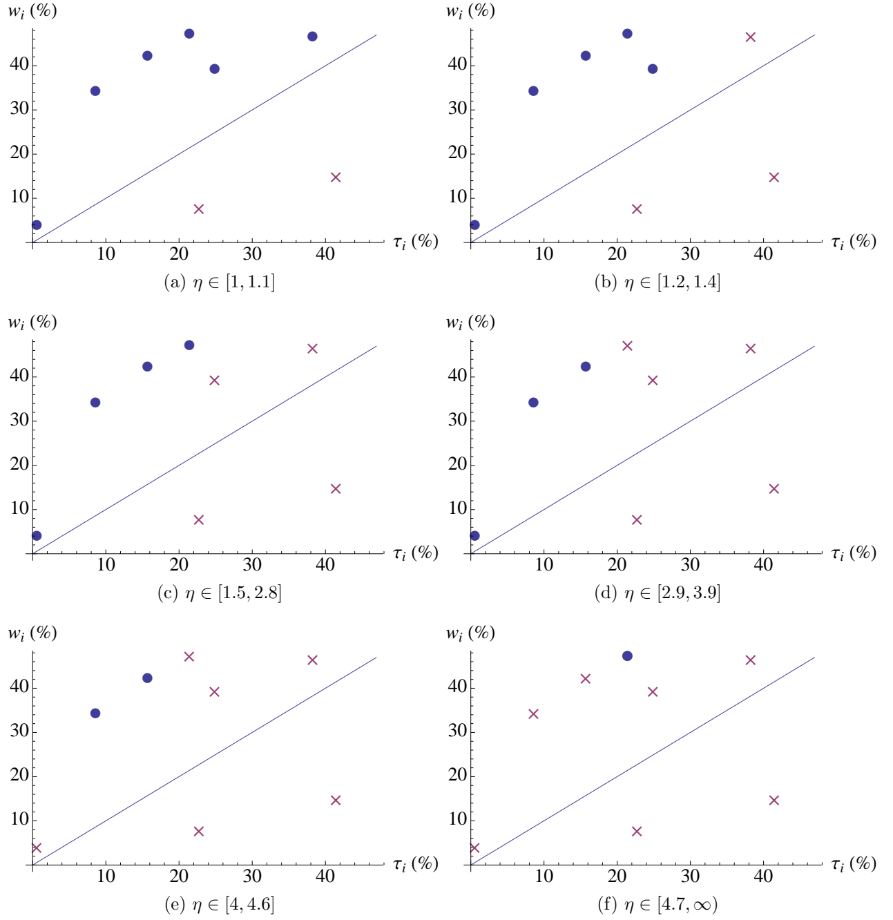
Figure 5: Large catastrophes. Optimal project choice at different levels of risk aversion, \eta .
