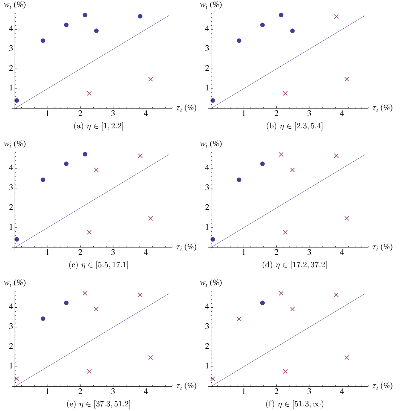
Figure 6: Small catastrophes. Optimal project choice at different levels of risk aversion, \eta .
