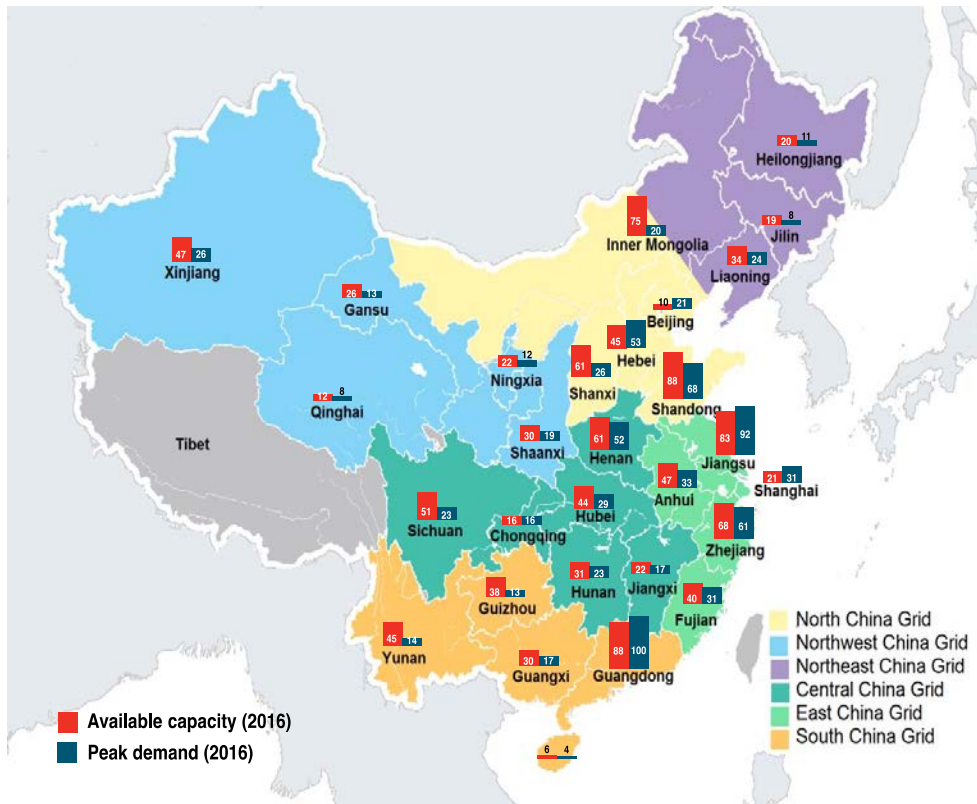
Available capacity versus peak demand by province, 2016 (GW)
