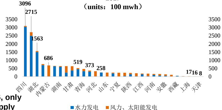
Provincial hydro, wind and solar power generation in 2017
