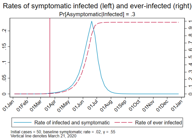
Figure 2. Policy path (A) with low (left) and high (right) asymptomatic rates
