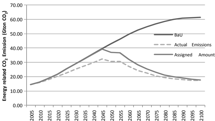
Figure 3(b). Targets and emission by developing countries under the 500 ppm goal
