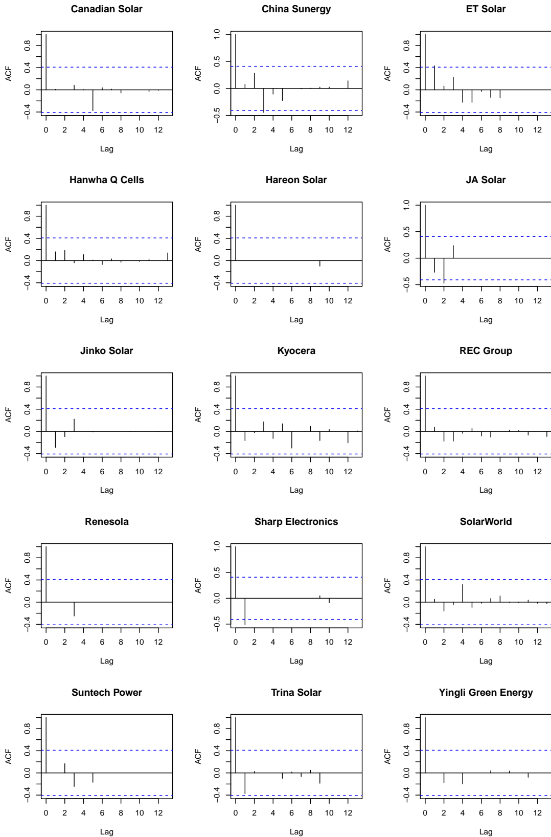
Figure D2: Autocorrelation of Investment Level ( v_{it} ) within a Firm
